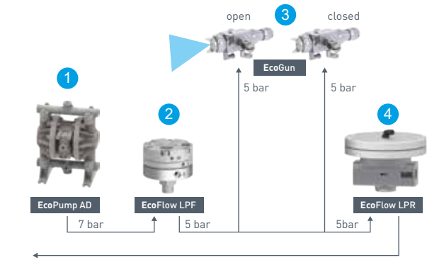
1 - Pump, 2 - Pressure flow regulator, 3 - Spray guns, 4 - Return flow regulator
