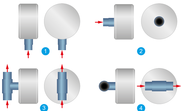
Pressure gauge connector positions
