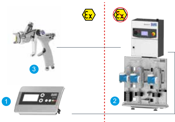
1 - EcoPUC, 2 - EcoDose 3K, 3 - EcoGun
